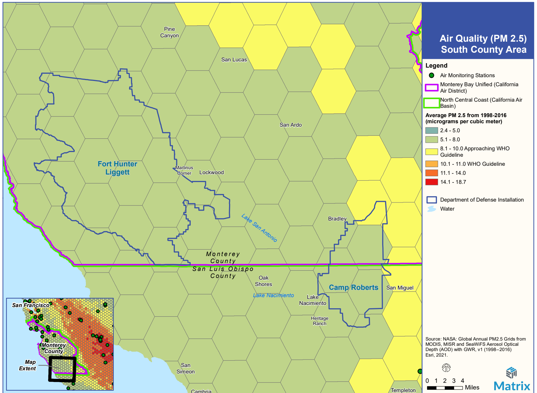
FigX-X_MRCUS_South_Air_Quality_2pt5_PM_2021_09_23_EBR.pdf
